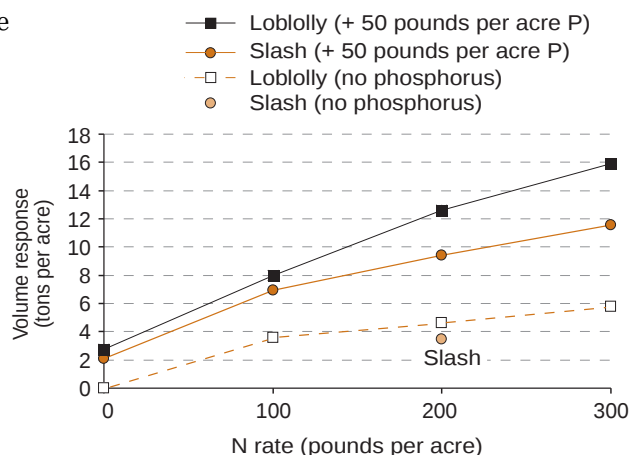
Figure 8.6—Growth response of loblolly and slash pine on a variety of soil types following midrotation application of nitrogen (N) and phosphorus (P) fertilizer (adapted from North Carolina State Forest Nutrition Cooperative 1997).
