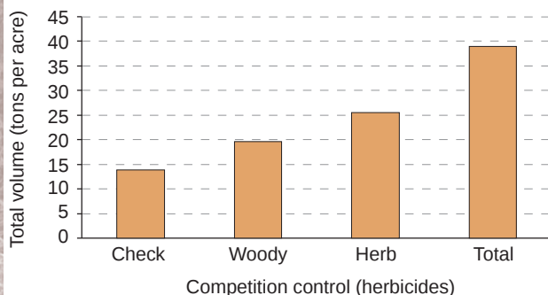
Figure 8.5—Effect of competition control on growth of loblolly pine at age 8 (adapted from Miller and others 1995).
